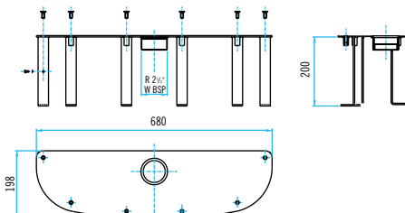
Anclaje ancho 600 mm Cod. 19985 600 mm wide anchor
