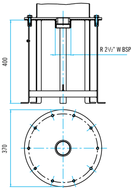
Anclaje circular Ø 254 Circular anchor Ø 254 Cod. 19984
